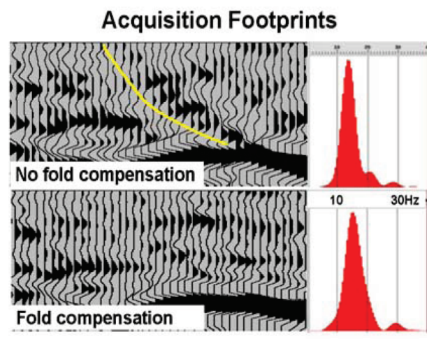
Fig. 4. Impulse response noise for data not pre-conditioned to compensate for surface sampling irregularity. The spectrum of the compensated data is broader in this case (but not always).
