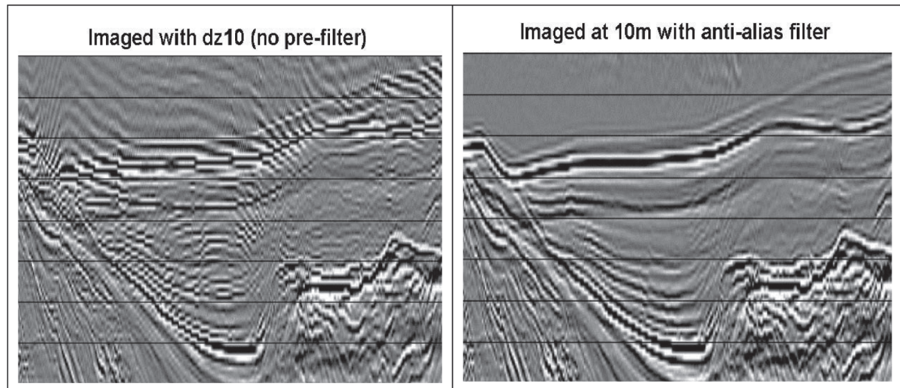
Fig. 2. Effects of not compensating for depth-temporal aliasing in the migration
