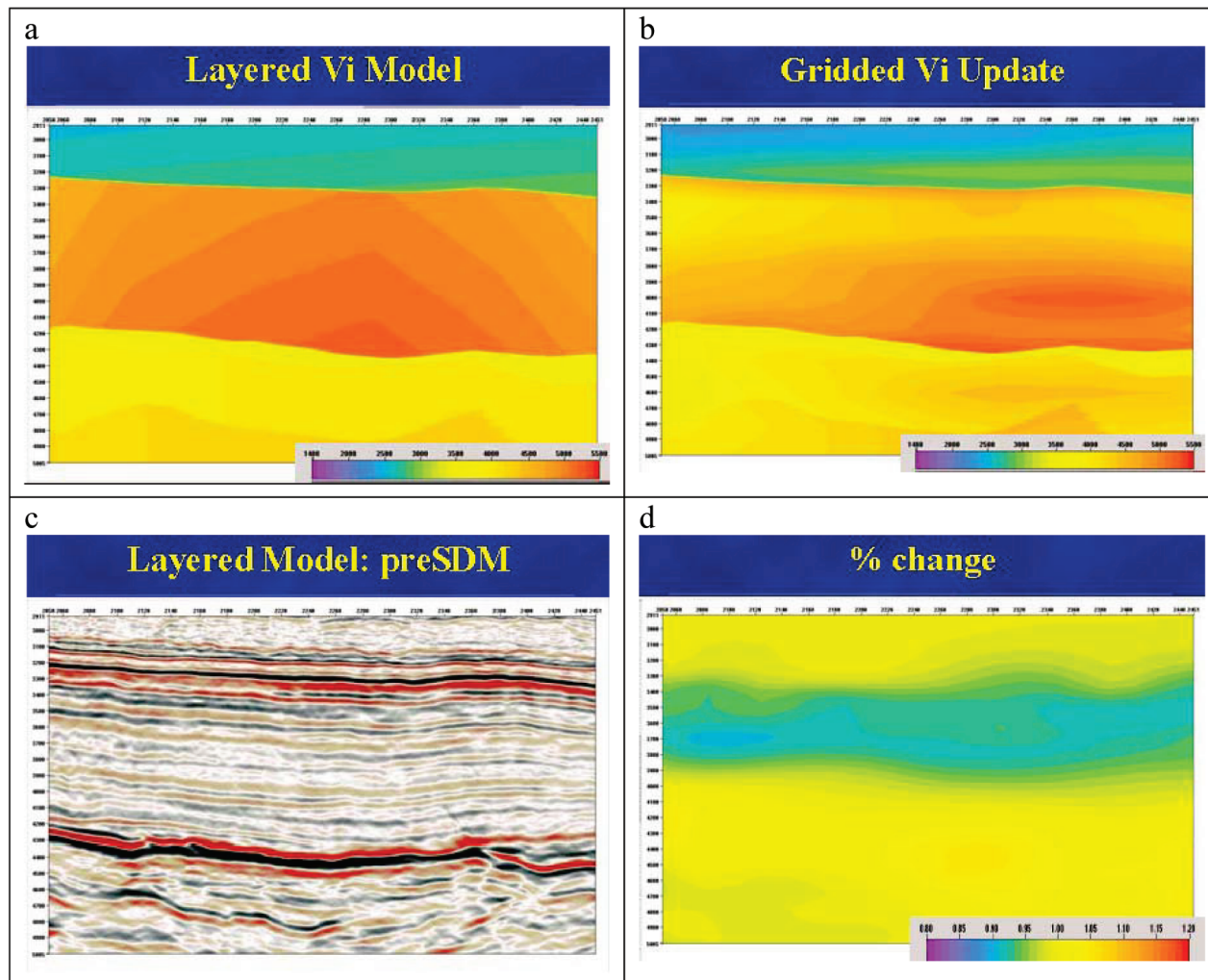
Fig. 1. a: layered model with vertical compaction gradients in the chalk, b: the gridded update, c: the PreSDM from the layered model, d: the percentage change in velocity resulting from the gridded update
